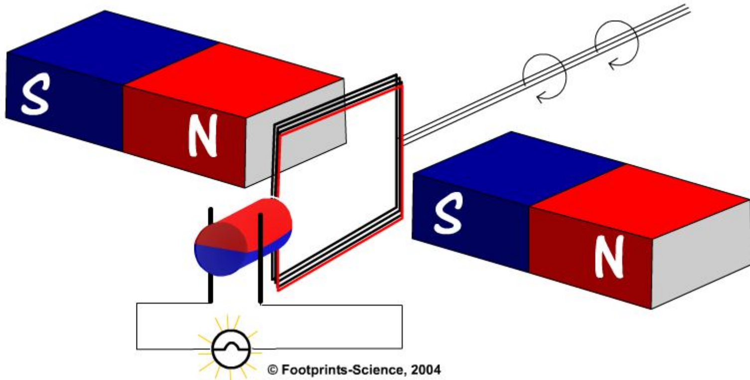
Generator
